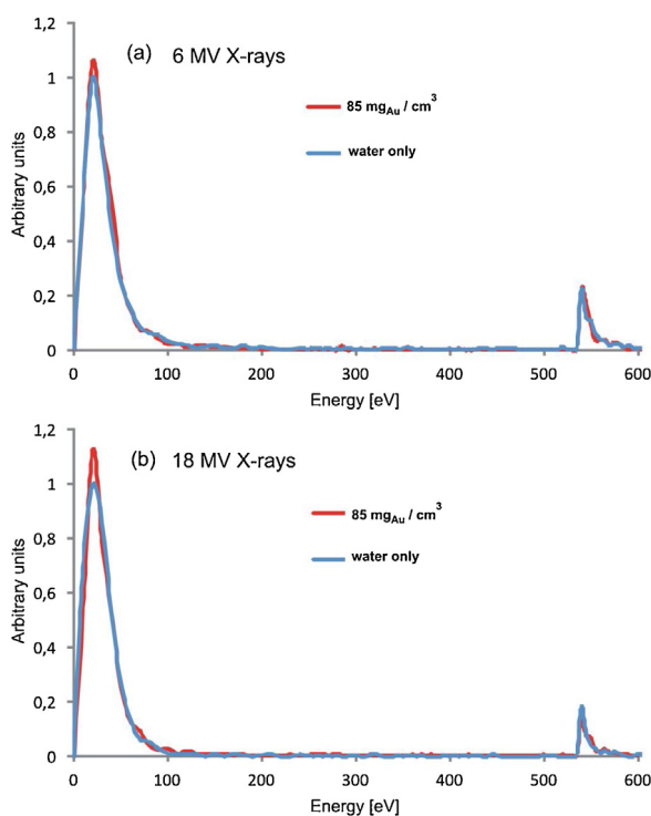
Fig. 4. The spectra of energy absorbed in water in the nanophantom with and without 2D AuNPs for the gold mass concentration of 85 mg Au /cm 3 for 6 MV X-rays (a) and for 18 MV X-rays (b). The events were counted in the 10 eV bins up to 250 eV and in the 5 eV ones for the higher energies. The counts in the bins were normalized to the maximum of the spectra without AuNPs.
