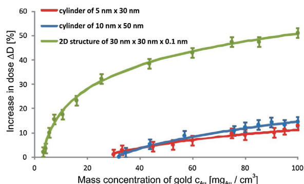
Fig. 3. The increase of the dose absorbed in water in the target volume irradiated by 18 MV X-rays versus the mass concentration of gold for AuNPs with the considered shapes and sizes. Otherwise as in Fig. 2.
