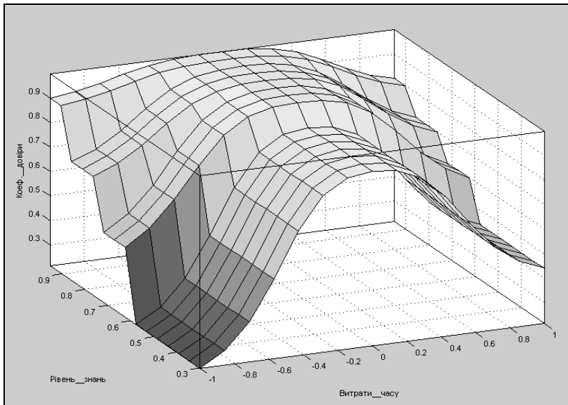
Figure 3. The surface of the fuzzy output for the value of the coefficient k_s Source: Own work
